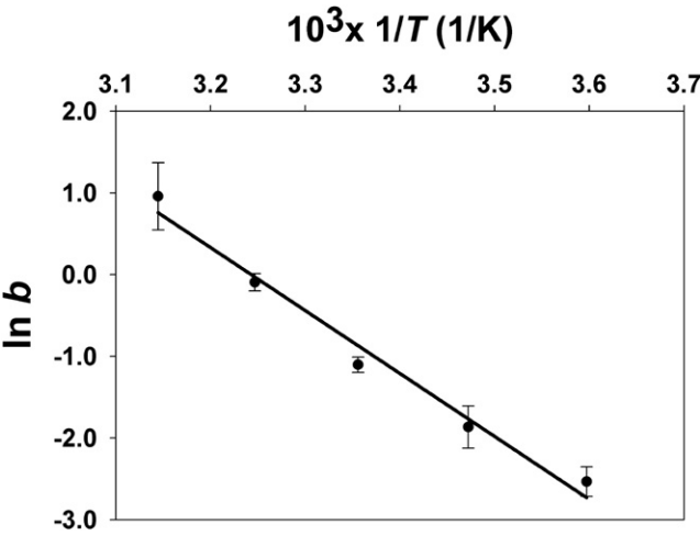
FIGURE 6 Effect of temperature on 16AP transfer from YLSACP2 to membranes. Transfer of 16AP from a preformed complex, prepared by incubating 0.25 \mu M 16AP with 2.5 \mu M YLSCP2, to 150 \mu M NBD-containing zwitterionic EPC-SUV was monitored at 10°C intervals from 5 to 45°C. The data were analyzed as described in Materials and Methods . Transfer rates (mean \pm SE) from three separate experiments are shown in the Arrhenius plot, where b is the transfer rate ( r^2 = 0.98 ).
